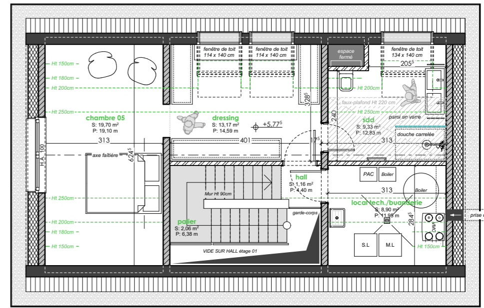
Combles
